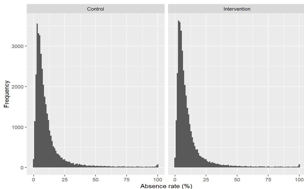
Figure 3: Distribution of absence rate (%) across Terms 2–6 (primary outcome), by trial arm
